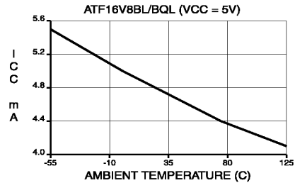
SUPPLY CURRENT vs. AMBIENT TEMPERATURE
