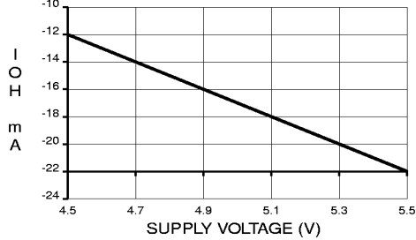
OUTPUT SOURCE CURRENT vs. SUPPLY VOLTAGE (TA = 25C)
