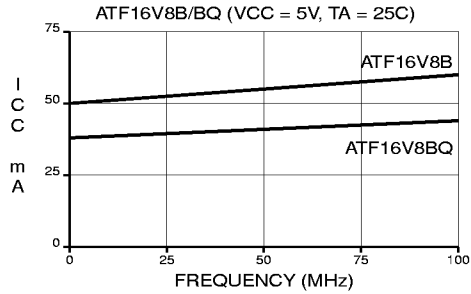
SUPPLY CURRENT vs. INPUT FREQUENCY
