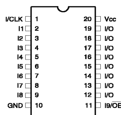
DIP/SOIC
