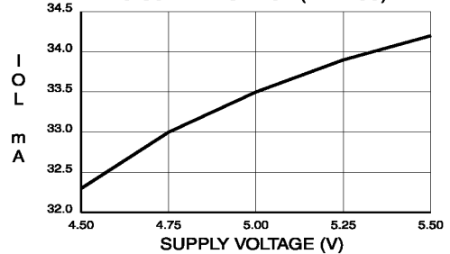
OUTPUT SINK CURRENT vs. SUPPLY VOLTAGE (TA = 25C)
