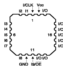
PLCC Top View
