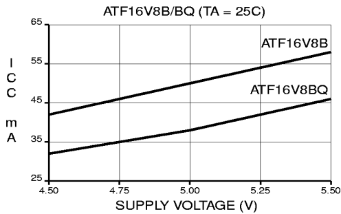
SUPPLY CURRENT vs. SUPPLY VOLTAGE
